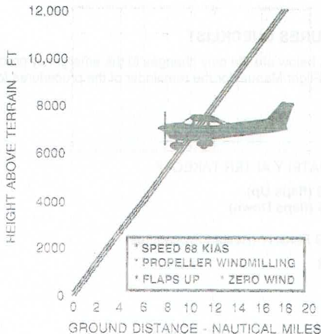
Figure 4 Maximum Glide
